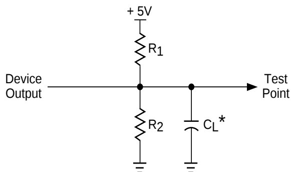
Figure 3. Test Load
